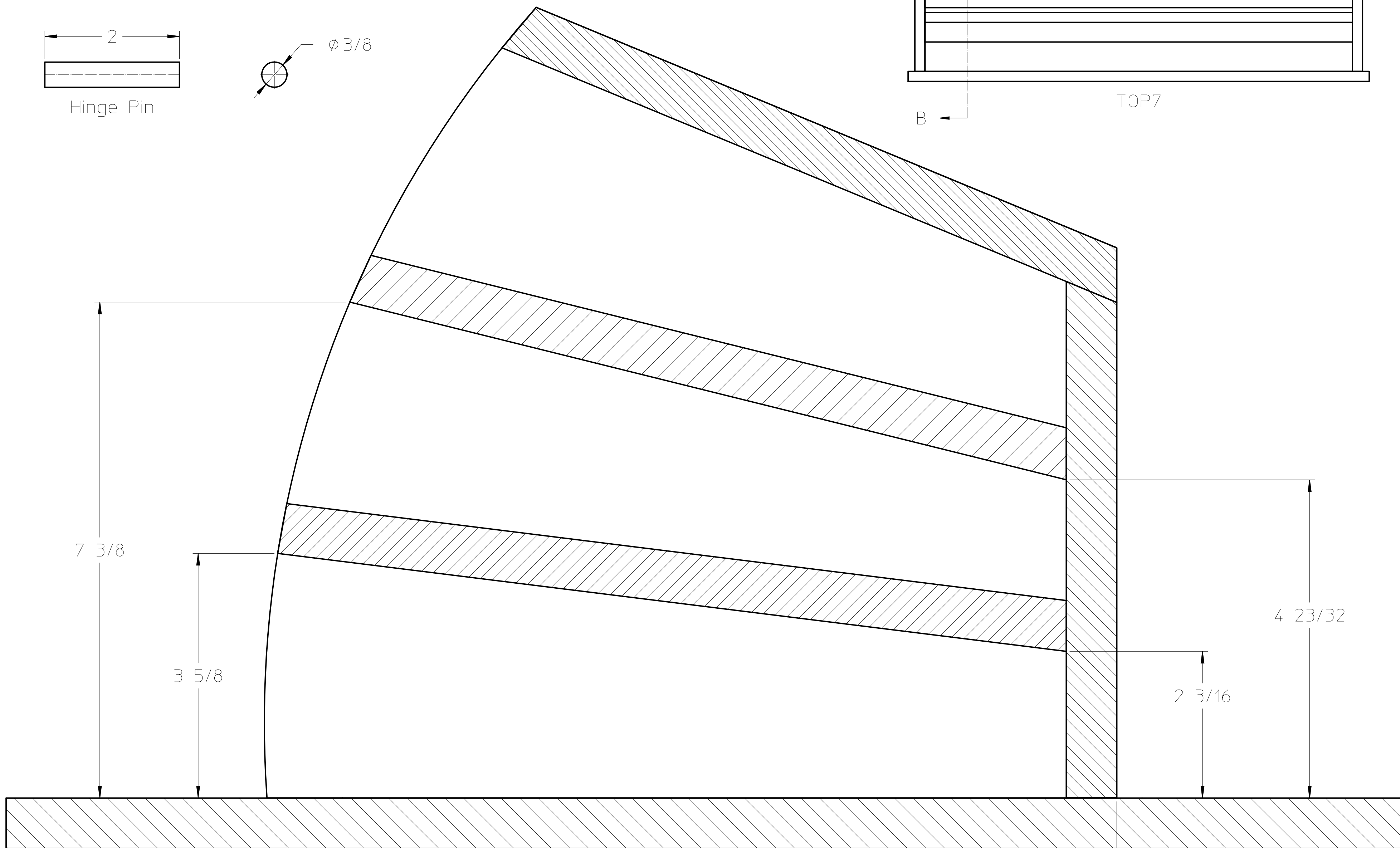
Shoe Shelf Section B-B
